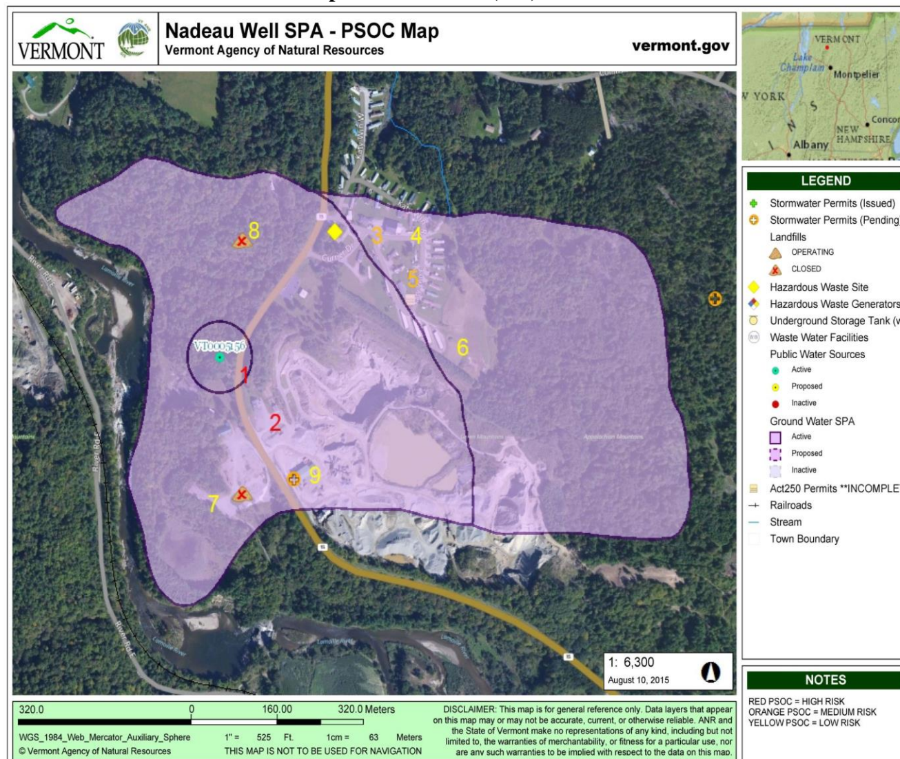
Figure 4. Potential Sources of Contamination Map – Nadeau Well (001)
